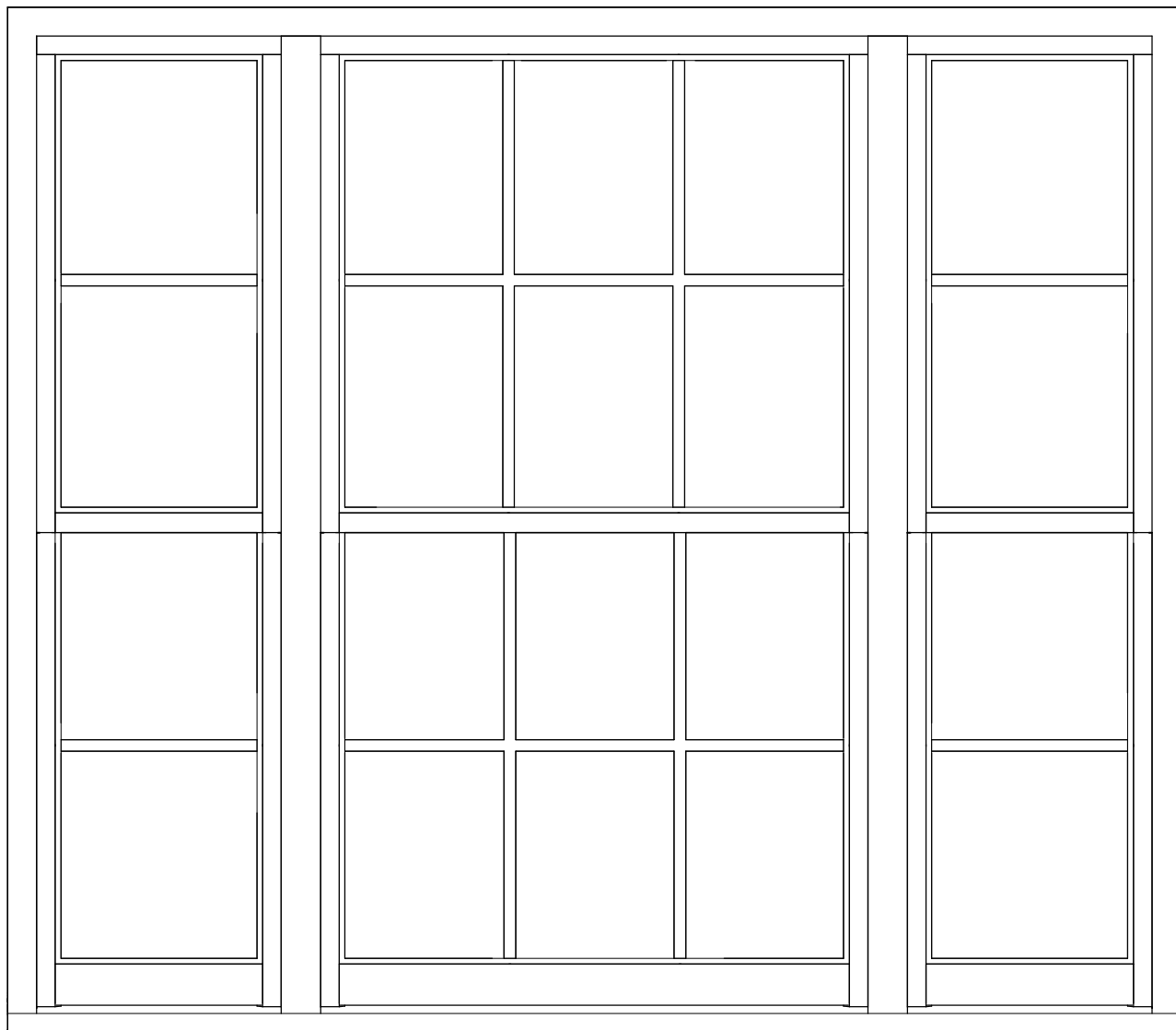
02 Front View 1 : 12
