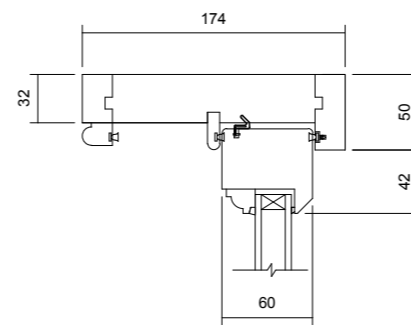
05 Head Detail 1 : 5
