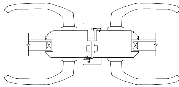
05 Meeting Stile 1:5
