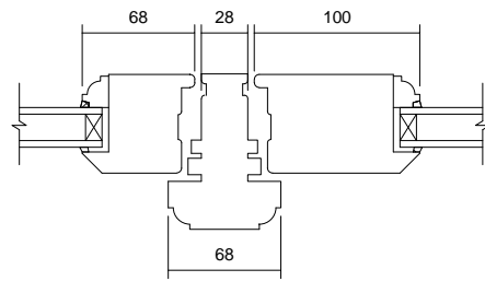
04 Mullion Detail 1:5
