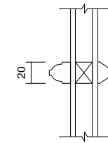
07 Glazing Bar Detail 1:5
