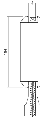
06 Mid Rail Detail 1 : 5
