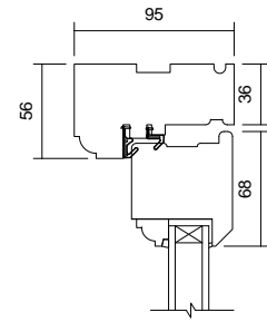
05 Head Detail 1 : 5
