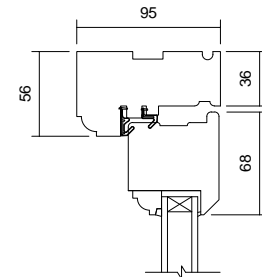
05 Head Detail 1 : 5
