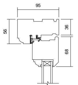
05 Head Detail 1 : 5
