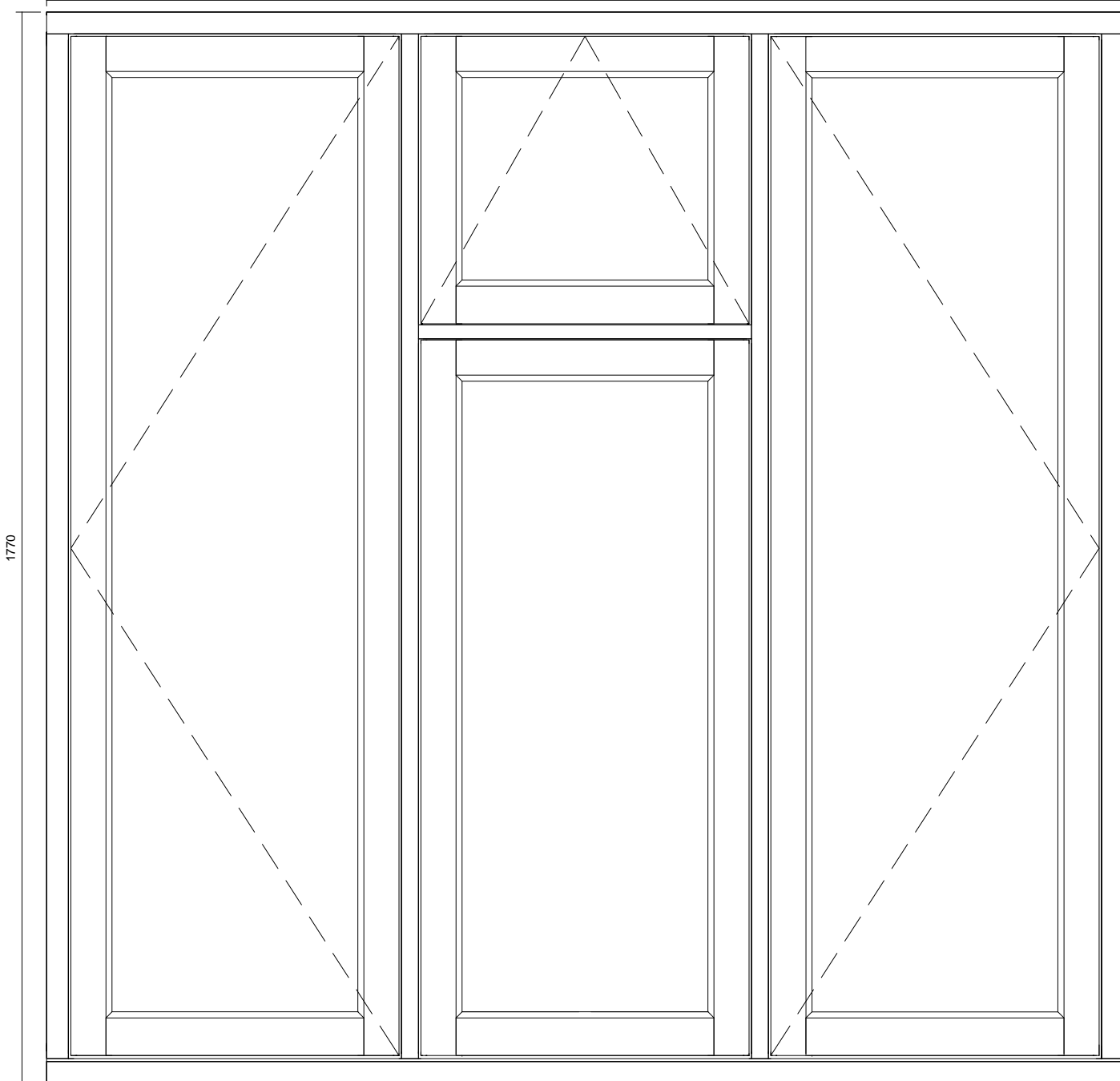
02 Front View 1 : 10
