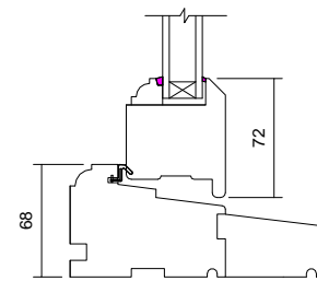
06 Cill Detail 1 : 5
