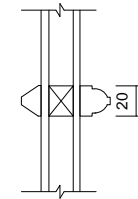
05 Glazing Bar Detail 1 : 5
