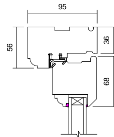
04 Head Detail 1 : 5
