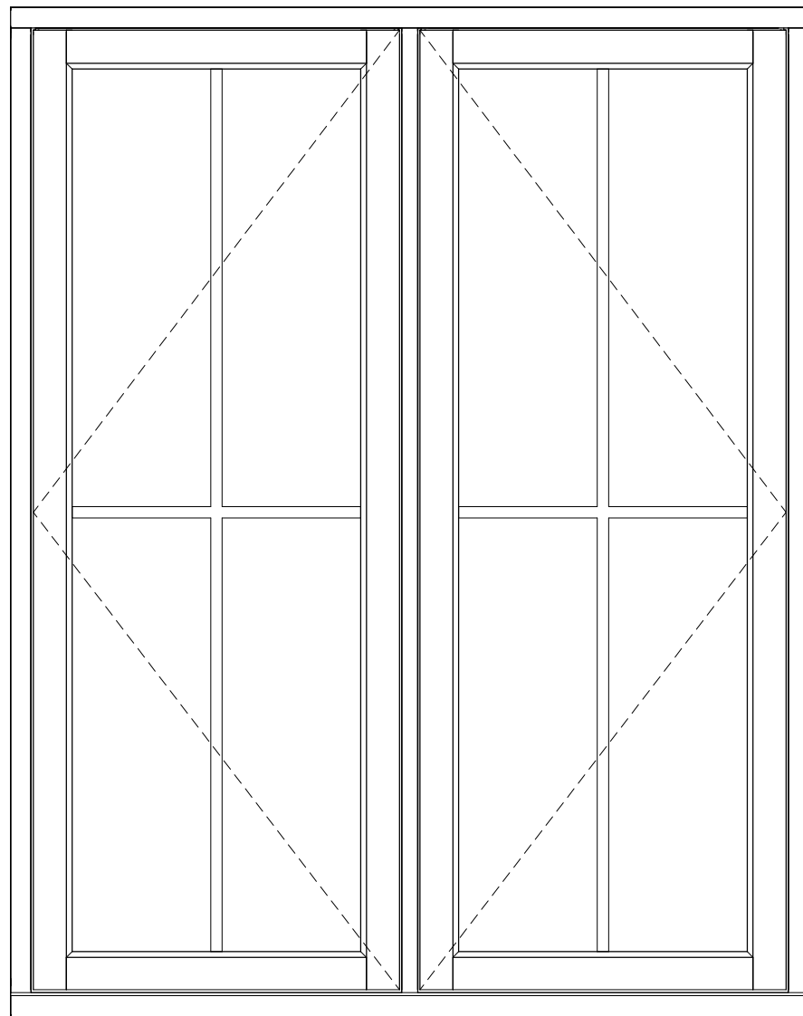
02 Front View 1 : 12
