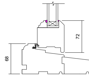
06 Cill Detail 1 : 5
