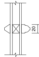
05 Glazing Bar Detail 1 : 5
