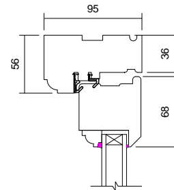
04 Head Detail 1 : 5
