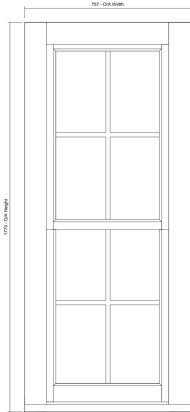
02 Front View 1 : 10
