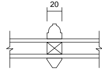
04 Glazing Bar Detail 1 : 5
