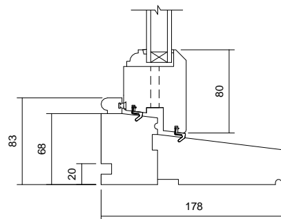
07 Cill Detail 1 : 5
