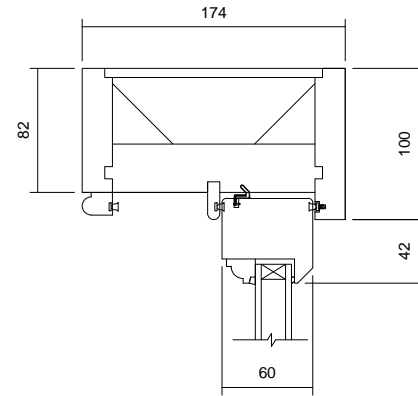
05 Head Detail 1 : 5
