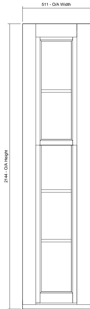
02 Front View 1 : 15
