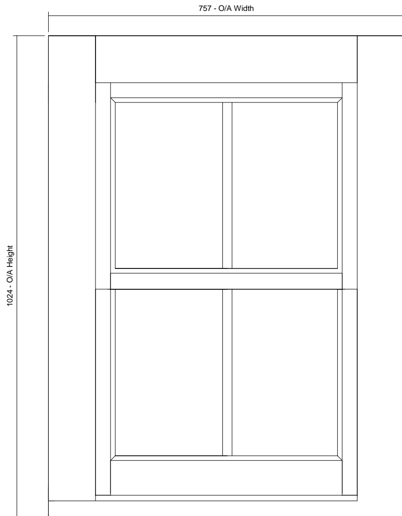
02 Front View 1 : 8
