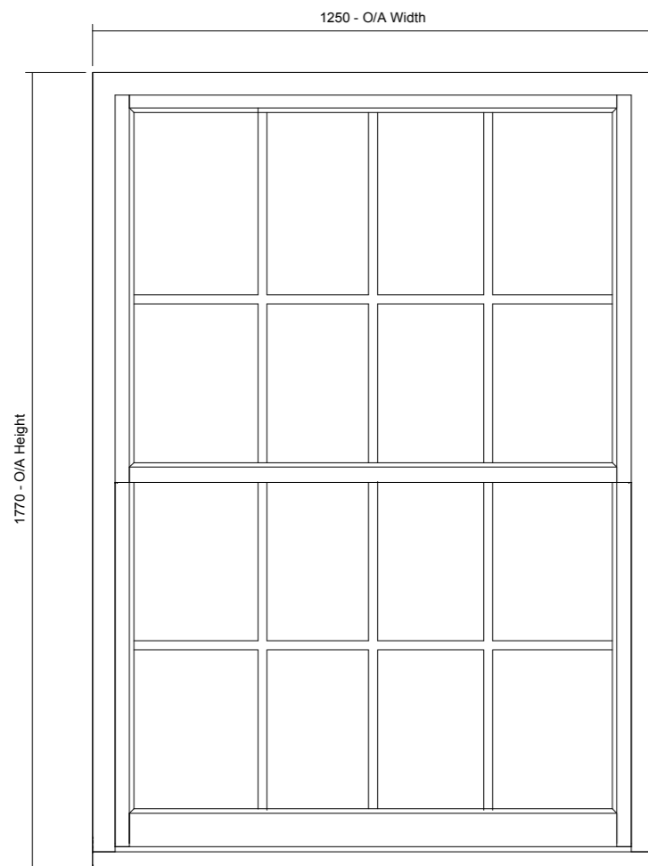
02 Front View 1 : 15
