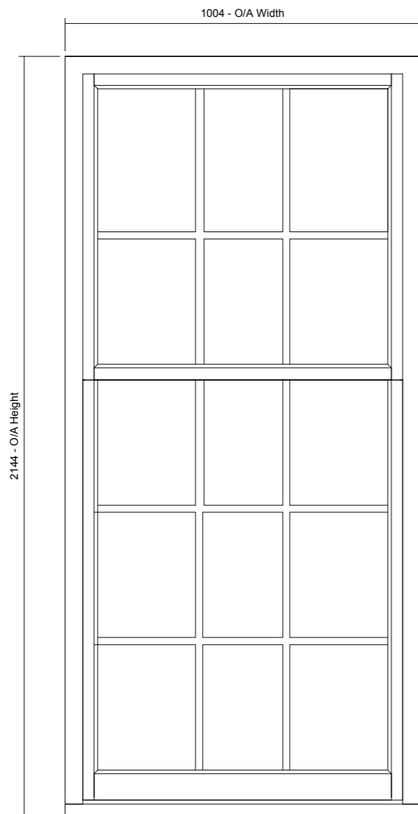
02 Front View 1 : 15
