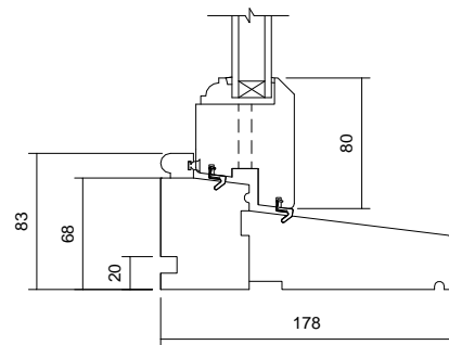
07 Cill Detail 1 : 5
