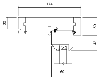
05 Head Detail 1 : 5
