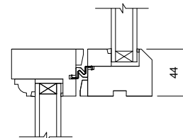
06 Meeting Rail Detail 1 : 5
