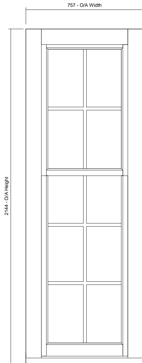
02 Front View 1 : 15
