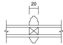
04 Glazing Bar Detail 1 : 5
