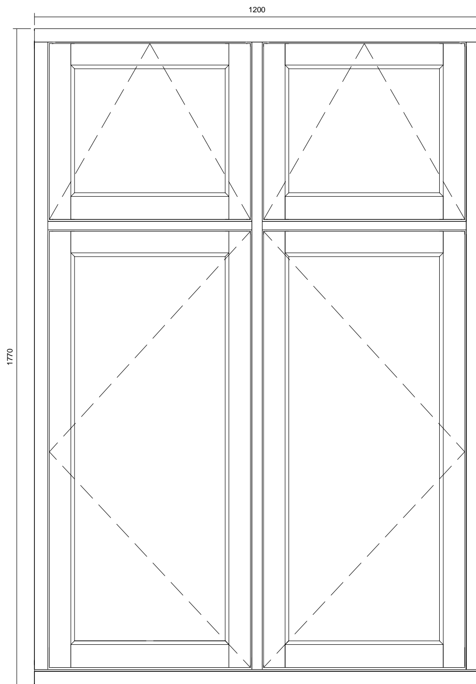
02 Front View 1 : 10
