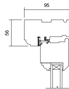
05 Head Detail 1 : 5
