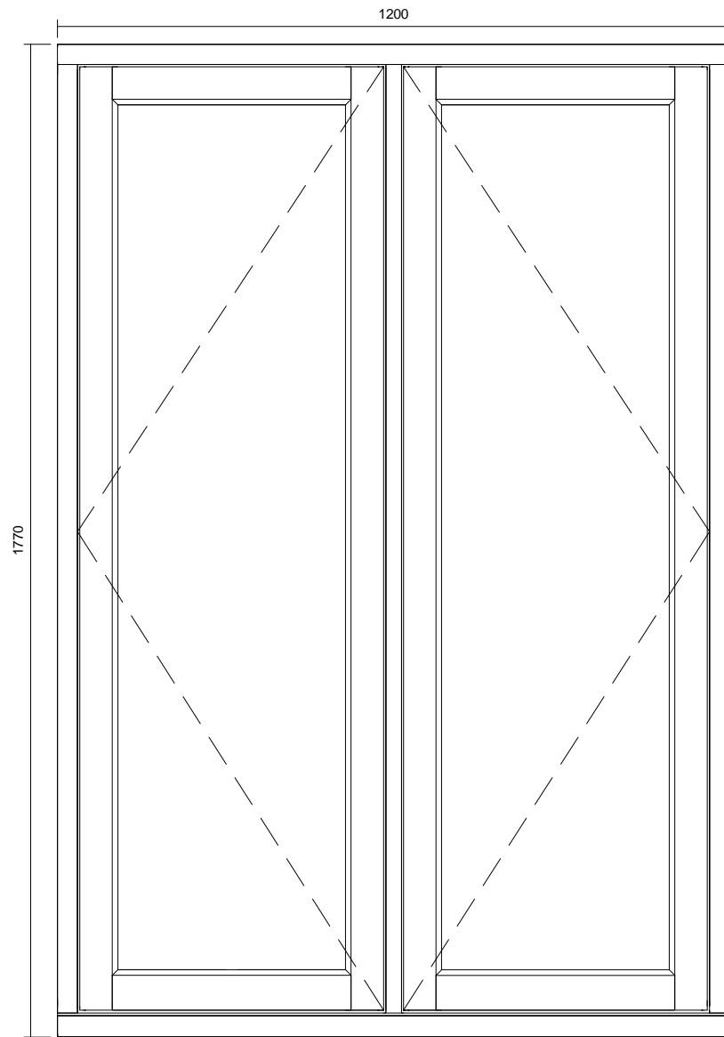
02 Front View 1 : 12
