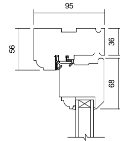
06 Head Detail 1 : 5
