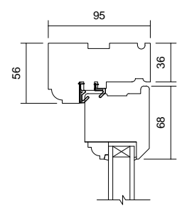
04 Head Detail 1 : 5
