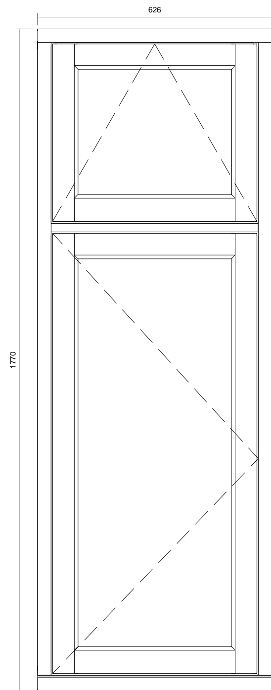
02 Front View 1 : 10
