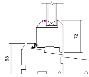
06 Cill Detail 1 : 5
