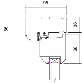
04 Head Detail 1 : 5
