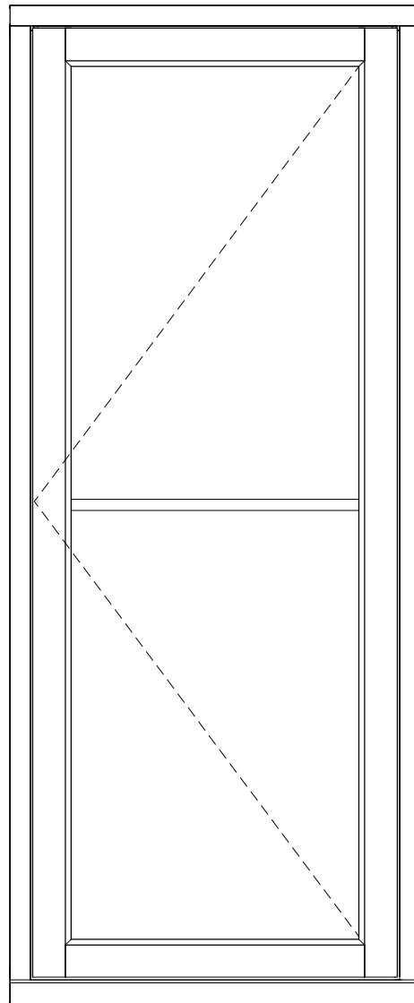
02 Front View 1 : 12
