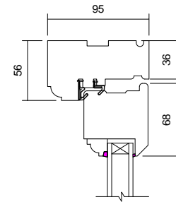
04 Head Detail 1 : 5
